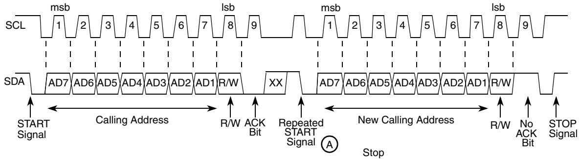
Figure 24-3. Repeated START
